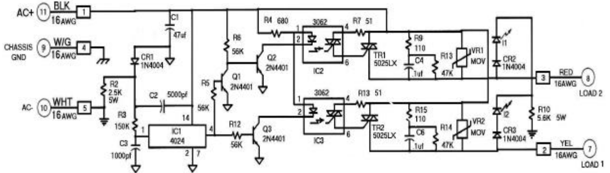
SCHEMATIC DIAGRAM
